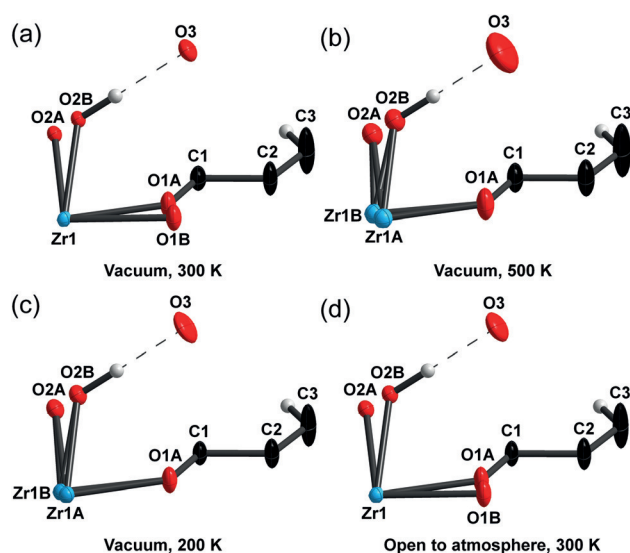
Figure 4. Asymmetric unit of UiO-66 measured in the environment cell. The measurement begins at room temperature under vacuum (a, UiO-66_GC1), then heated to 500 K at 200 K h -1 (b, UiO-66_GC2), during which the water molecules replacing the linker are removed to leave open metal sites on Zr. The crystal was then cooled to 200 K (c, UiO-66_GC3) for a more accurate structure determination. Finally, the crystal was warmed to room temperature and exposed to the atmosphere (d, UiO-66_GC4), where the water molecules are once again coordinated to Zr. Ellipsoids are shown at 50% probability.
